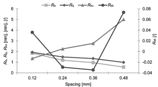
Fig. 3. Surface roughness parameters in dependence of spacing between dimples (diameter of dimples 0.12mm, depth 6 \mu m)
