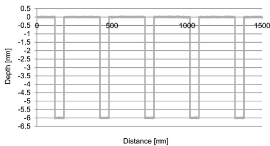
Fig. 2. Example of virtually textured surface (diameter of dimples 0.06 mm, spacing 0.24 mm, depth 6 \mu m, rectangular shape)
