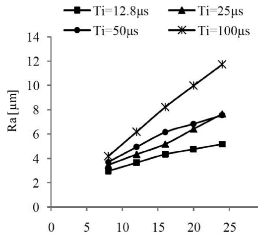
Fig. 9. R_a vs. pulse current
