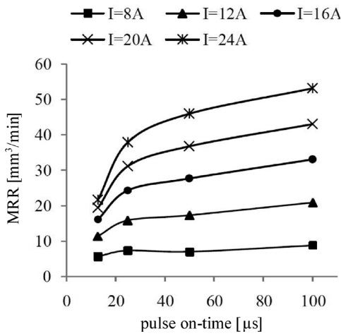
Fig. 4. MRR vs. pulse on-time
