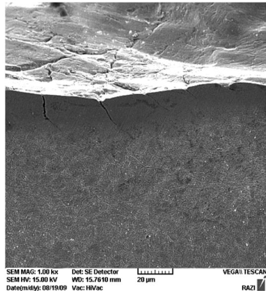
Fig. 3. SEM micrograph showing the white layer of EDMed workpiece ( I = 24 A and T_i = 100 \mu s )
