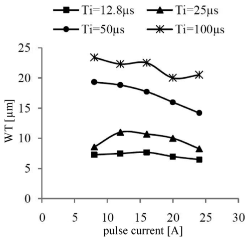
Fig. 12. WT vs. pulse current
