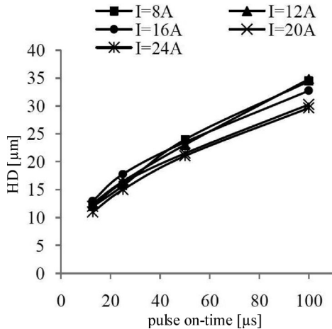
Fig. 11. HD vs. pulse on-time
