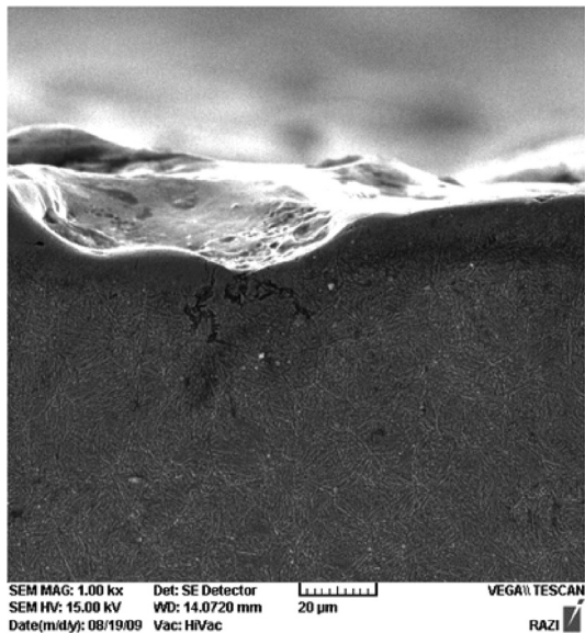
Fig. 2. SEM micrograph showing the white layer of EDMed workpiece ( I = 24 A and T_i = 50 \mu s )
