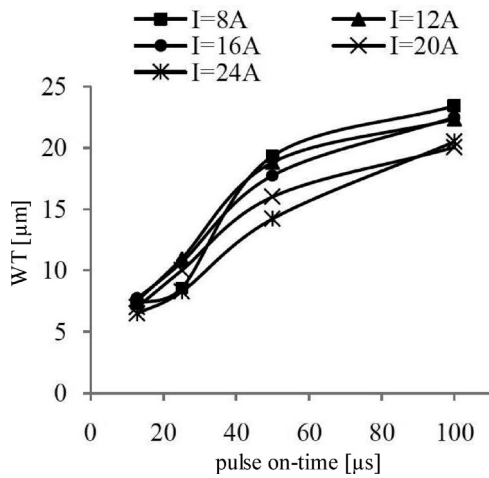
Fig. 10. WT vs. pulse on-time
