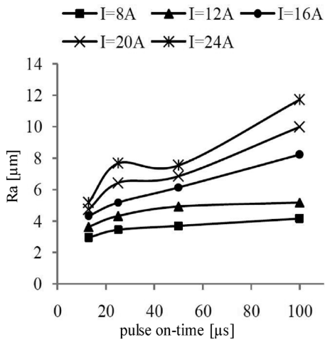
Fig. 6. R_a vs. pulse on-time
