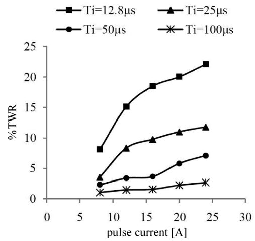
Fig. 8. TWR vs. pulse current
