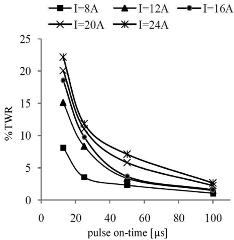
Fig. 5. TWR vs. pulse on-time
