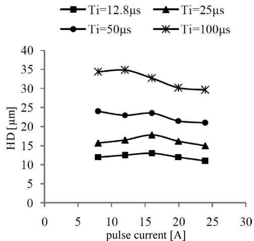
Fig. 13. HD vs. pulse current
