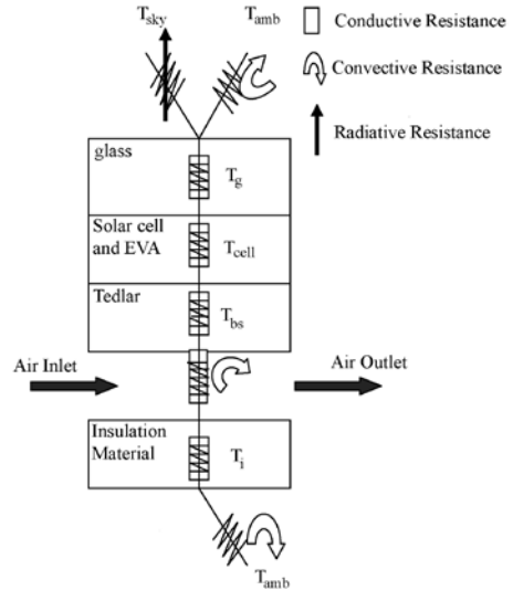
Fig. 1. The equivalent thermal resistant circuit of a PV/T air collector [5–9]
