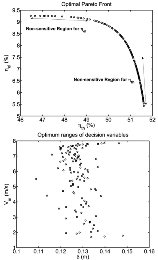
Fig. 9. The optimum values of objective functions and decision variables in optimal Pareto front
