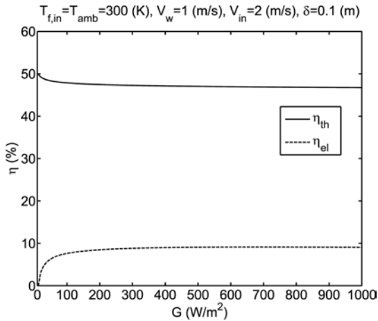
Fig. 12. The effect of solar radiation intensity on the thermal efficiency and electrical efficiency
