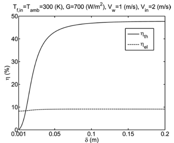
Fig. 11. The variations of thermal efficiency and electrical efficiency with respect to duct depth
