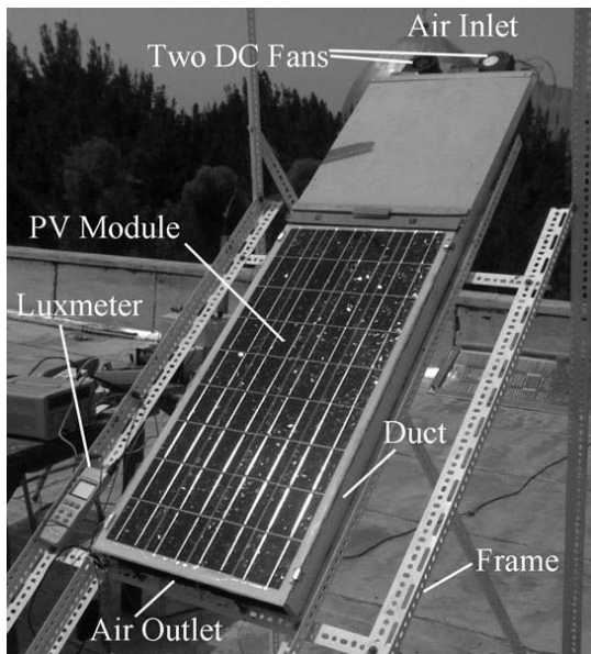
Fig. 4. Photograph of experimental setup of hybrid PV/T air collector at Zahedan (Iran)
